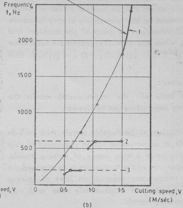
Fig.5. Laws of chatter formation during metal cutting process
