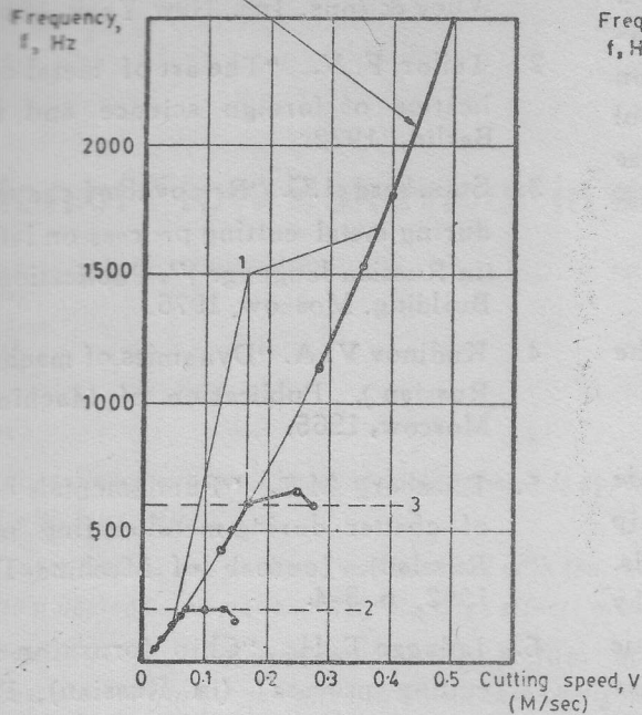
Fig.5. Laws of chatter formation during metal cutting process
